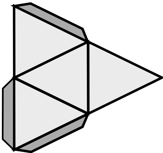
i.) Tetrahedron
